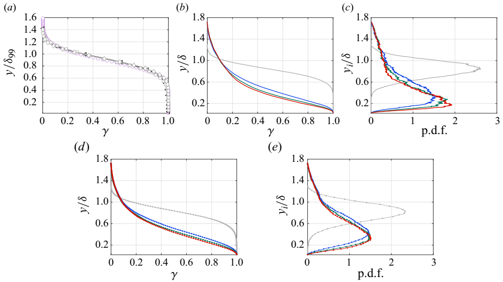
Figure 7. (a) Intermittency profiles for case |\omega^*| = 0.2 from Borrell & Jiménez (2016) ( -\triangleleft- , black), case s_{th} = 40 from Reuther & Kähler (2018) ( \circ , violet) and case REF of the present study obtained using the velocity interface ( -\diamond- , grey) and the vorticity interface ( -\blacksquare- , grey). (b,d) Intermittency profiles and (c,e) p.d.f.s of the interface location for cases A (blue), B (green) and C (red) measured at X/M = 55 as well as case REF (grey), with (b,c) derived using the velocity interfaces and (d,e) derived using the vorticity interfaces.
