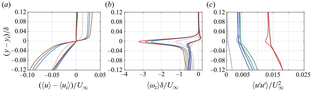
Figure 9. (a) Streamwise velocity, (b) spanwise vorticity and (c) streamwise turbulent fluctuations profiles conditionally averaged across the velocity interface (—) and the vorticity interface (— • —) for cases A (blue), B (green) and C (red) measured at X/M = 55 as well as case REF (grey).
