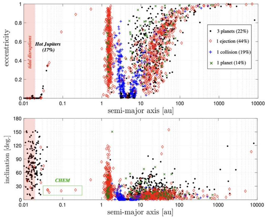
Figure 1. The final orbital elements after 10 Myrs for three-planet systems, where the majority ( \simeq 95\% ) undergoes a phase of strong gravitational scattering. The symbols indicate various outcomes (see Table 1 for more details). A significant population of hot Jupiters is formed, the majority in systems where all 3 planets remain in the system. Note, however, that these planets would have likely been disrupted as their pericenter distances reach inside \simeq 2R_\odot (shaded region in red). In turn, hot Jupiters in two-planet systems tend to circularize to wider orbits, some of which are driven by Coplanar High-eccentricity Migration (CHEM; see green box in lower panel and an example in Figure 2).
