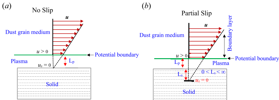
FIGURE 6. A schematic diagram of dusty plasma flow around a solid surface. (a) No slip and (b) partial slip. The potential boundary is separating the plasma and dust-grain medium. Length L_p is the length of the plasma column or sheath dimension or void dimension over the solid surface.
