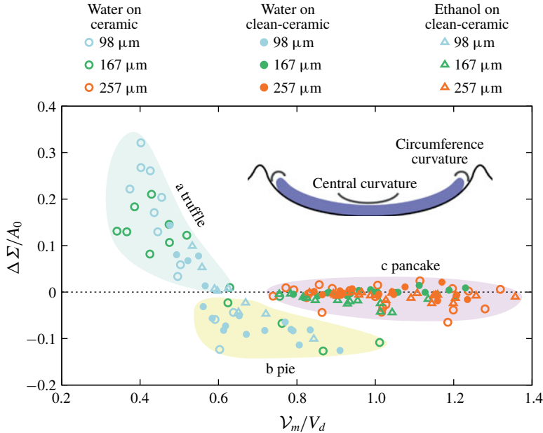
FIGURE 3. (Colour online) Main plot: crater area difference, \Delta\Sigma , plotted versus the estimated mixing ratio \mathcal{V}_m/V_d . The sign of \Delta\Sigma , here normalized by the corresponding flat area A_0 , indicates the final morphology. The morphology develops with the estimated mixing ratio \mathcal{V}_m/V_d . Three regimes can be distinguished which are in accordance with the residue morphology shown in figure 1: a, truffle; b, pie; c, pancake. See text for details and for the definition of \Delta\Sigma and A_0 . Inset: a sketch of the two curvatures occurring in a spread droplet. In practice, the droplet (blue) is mixed with grains which are not drawn here.
