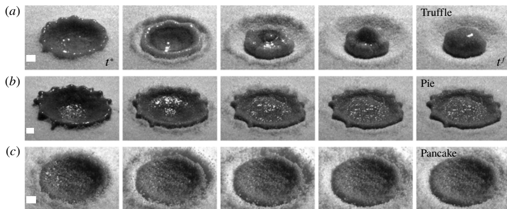
FIGURE 1. The formation of three morphologies; (a) truffle, (b) pie and (c) pancake. Each row represents five consecutive snapshots of an impact. The leftmost snapshot is at the moment of reaching the maximum expansion of the droplet, t = t^* (namely, t^* = 5.2 ms, 5.6 ms and 5 ms, respectively from top to bottom). The rightmost one is the last frame, t = t^f , showing the final steady state. The snapshots in between correspond to t^* + 5 ms, t^* + 10 ms, t^* + 15 ms. In each row snapshots are taken from the same viewpoint. Scale indicators of 1 mm by 1 mm are given at the left bottom in the leftmost image of each row.
