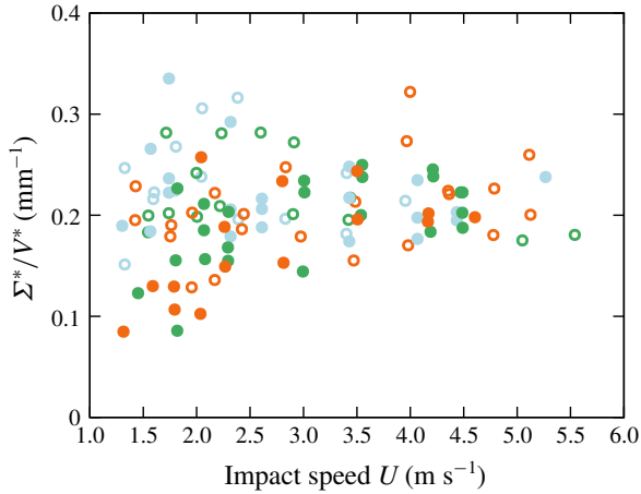
FIGURE 8. (Colour online) The ratio of the area and volume \Sigma^*/V^* is measured from the experimental profile at t^* . The scattering for a given U reflects the influence of the varying packing fraction of the granular target.
