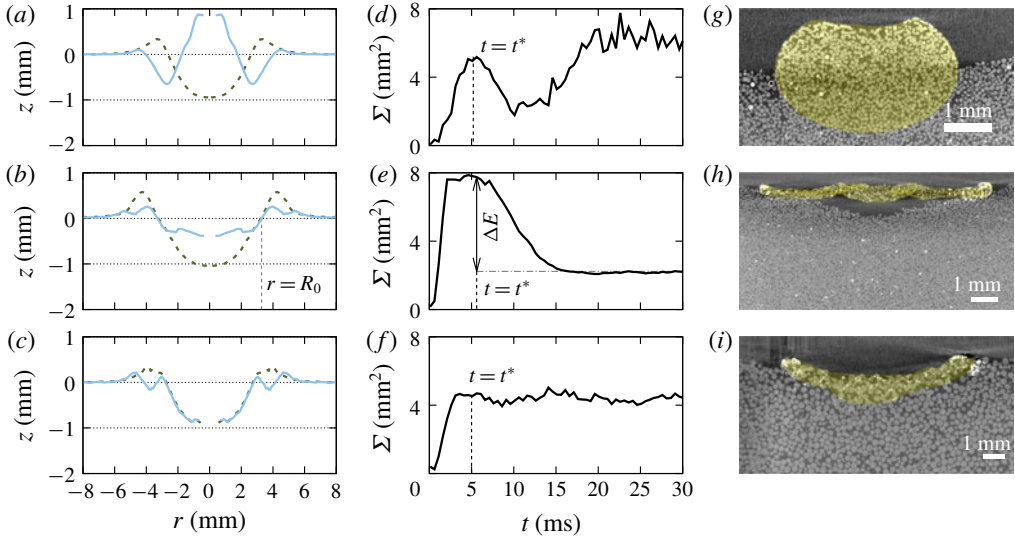
FIGURE 2. (Colour online) The leftmost column ( a–c ) illustrates the crater profile at the moment of maximal droplet expansion t = t^* (dashed lines) and the moment the final static state of the crater is reached, t = t^f (solid lines). For ( a, b ), the differences of crater profiles at these two moments result from the deformation of the liquid–grain mixtures, whereas the discrepancy at the crater rim in ( c ) is caused by grain splashing. The middle column ( d–f ) shows the time evolution of crater area, \Sigma (see text for definition). The moment t^* of maximum droplet expansion is indicated by vertical dashed lines in ( d–f ). In ( e ) the dash dotted line denotes \Sigma(t^f) . Both columns correspond to the impacts in figure 1. The rightmost column ( g–i ) displays vertical cross-sections from X-ray tomograms through the impact centre where the residual is highlighted with yellow colour. These tomograms are scanned for droplet impacts on glass beads, different experiments from that in ( a–f ). Details can be found in appendix A.
