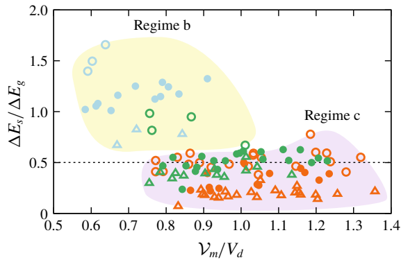
FIGURE 5. (Colour online) The data in regimes b and c in figure 3 are plotted versus the ratio of the virtual change of the surface energy, \Delta E_s , and the gravitational energy, \Delta E_g . See text for their definitions. The same symbols and colours as that in figure 3 are used here. The dashed line indicates the predicted lifting criterion, \Delta E_s / \Delta E_g = 0.5 , which separates the pie and pancake shapes in the overlapping range of mixing ratio.
