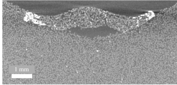
FIGURE 6. A vertical cross-section of a tomogram scan for water droplet impact on a packing of soda-lime beads. The impact speed, the grain size and the droplet size are the same as figure 2(h). However, the packing density is lower, namely equal to 0.55.
