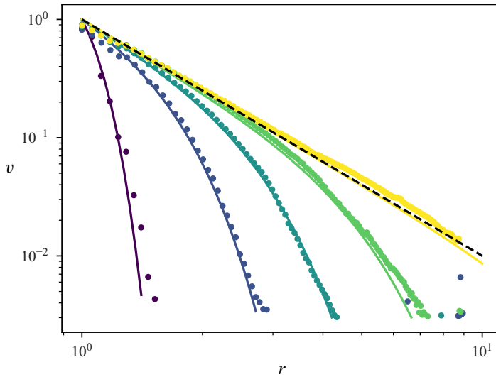
Figure 6. Theoretical and experimental azimuthal velocity radial profiles around a spinning sphere during spin-up. The velocities are measured and computed in the equatorial plane z = 0 . The dashed line is the theoretical stationary profile. The plots from dark to light correspond to the diffusive times t = 1.13 \times 10^{-2} , 2.25 \times 10^{-1} , 9 \times 10^{-1} , 3.6 and 65.61 . The circles are measurements from PIV. The lines are computed by the inverse Laplace transform. Here Ro = \infty , Re = 503 , Fr = 0.16 .
