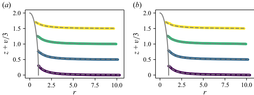
Figure 8. Theoretical and experimental azimuthal velocity radial profiles around a rotating prolate spheroid. Circles are PIV measurements. Each dashed line is the analytical base flow at that height; there is no fitting parameter. The base flow depends only on the aspect ratio. The profiles are shifted by their height and scaled by a factor of 1/3 to distinguish them. From dark to light, the heights are z = 0, 0.5, 1 and 1.5 with (a) Ro = \infty , Re = 670 , Fr = 0.320 , \Lambda = 2 and (b) Ro = 6 , Re = 838 , Fr = 0.288 , \Lambda = 2 .
