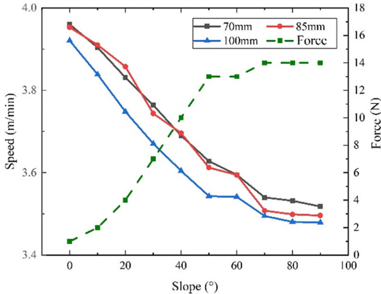
Figure 13. Slope-speed-force graph.
