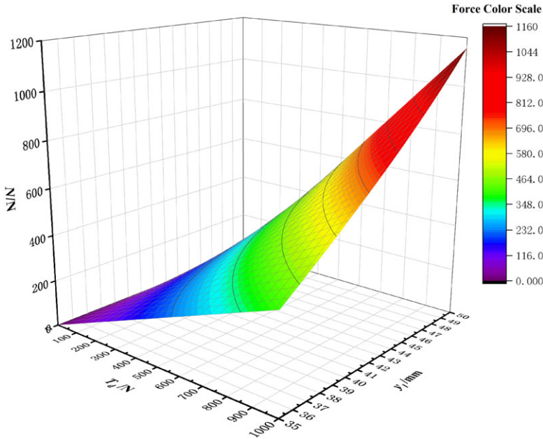
Figure 8. Relationship between thrust T_d , hole radius y_1 , and force N .
