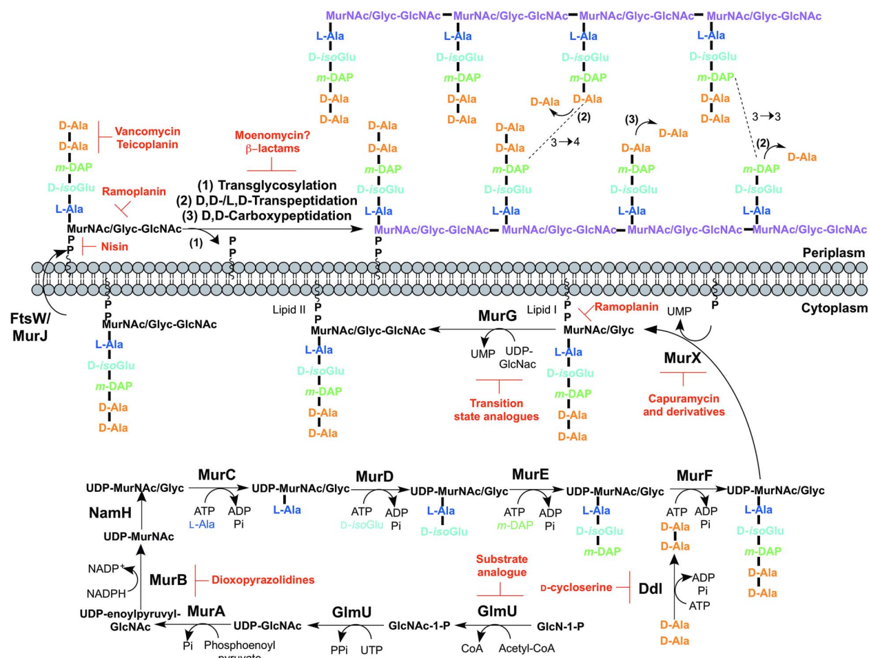
Fig. 2. Inhibitors targeting peptidoglycan biosynthesis. The roles of the key enzymes involved in peptidoglycan biosynthesis are illustrated. Reported inhibitors are shown in red.
