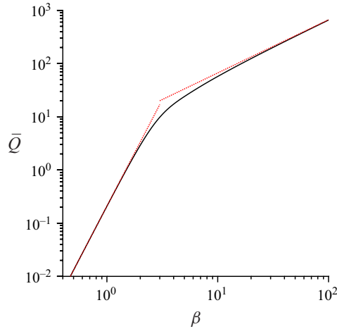
Figure 7. The non-dimensional heat generation rate per unit time \bar{Q} due to Joule heating as a function of \beta . The dotted red line on the left is the asymptotic expression (3.31) for \beta \ll 1 , and the dotted red line on the right is the asymptotic expression (3.32) for \beta \gg 1 .
