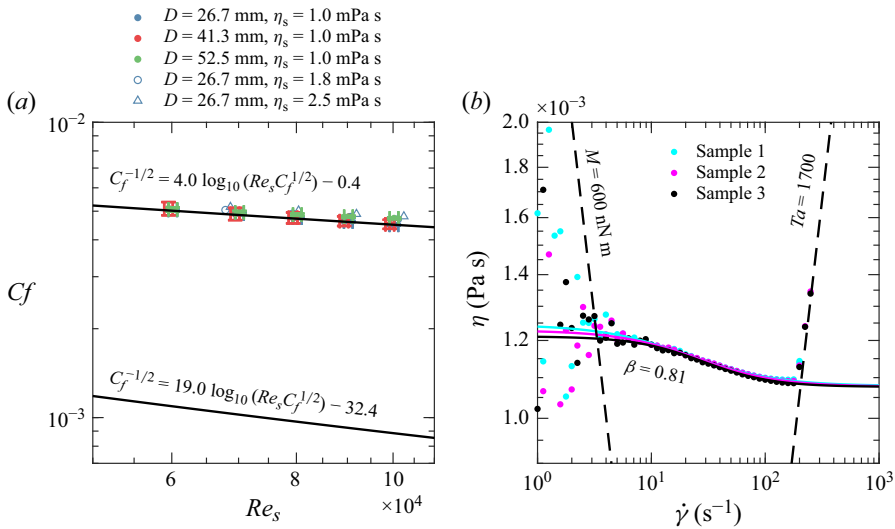
Figure 10. Plots of (a) C_f versus Re_s for Newtonian solvents in different pipe diameters D , and (b) repeated measurements of \eta versus \dot{\gamma} for a 50 ppm PAM solution. The upper and lower black solid lines in (a) are the skin-friction versus Reynolds number correlations for Newtonian turbulent pipe flow and MDR (Virk et al. 1970), respectively. Solid lines in (b) represent Cross model fits according to (2.1) and dashed black lines represent the low torque ( M > 600 nN m) and Taylor vortex ( Ta < 1700 ) limits of the viscosity measurements.
