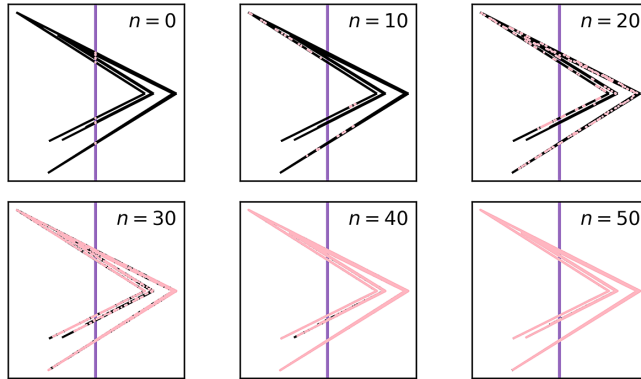
FIGURE 2. Exponentially fast filling of the Lozi attractor \Lambda \subset \mathbb{R}^2 (black) by the set intersection \Lambda \cap \{x = 0\} (pink), pushed forward n times by the same Lozi map. The level set \{x = 0\} is given in purple. Lozi parameters a = 1.8, b = 0.35 are used.
