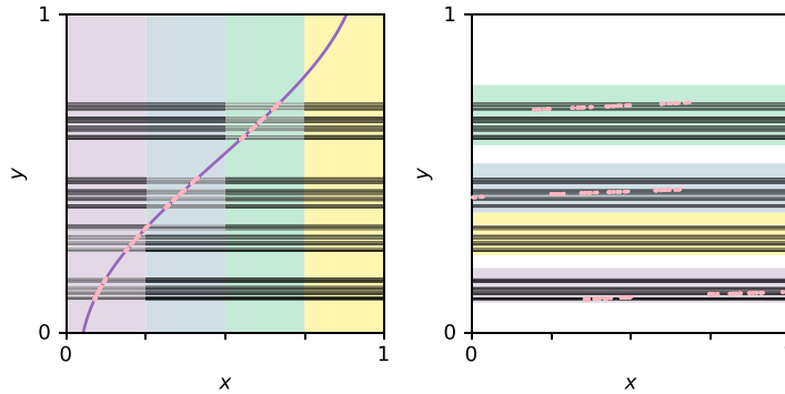
FIGURE 5. Picture of a baker’s map of the form (6) showing the attractor (black), an intersecting line x = \psi(y) - t_0 , a leaf of a transverse foliation of the form in Proposition 4.1, (purple), and the action of the map on pieces of the domain (in pale colours), and on the conditional measure of the SRB measure on the intersecting line (pink).
