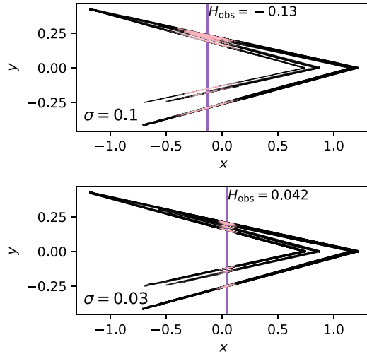
FIGURE 3. Posterior distribution (pink) after one observation step of H(u, v) = u + \zeta where \zeta \sim \mathcal{N}(0, \sigma^2) , for varying values of \sigma . Line corresponding to H(x, y) = H_{\text{obs}} in purple, attractor in black. Convergence to the conditional measure as in Figure 1 can be seen as the noise \sigma \rightarrow 0 .
