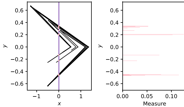
FIGURE 1. Left: picture of the Lozi attractor at a = 1.7 , b = 0.5 (black), the singular line \{x = 0\} (purple line), their intersection (pink Cantor set). Right: histogram of \rho(y | 0) , obtained from 200,000 iterates of the unstable manifold dynamics \bar{f} , binned at width 0.0025.
