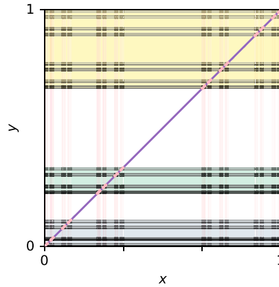
FIGURE 6. Picture showing the attractor [0, 1] \times C_{1/3} of the piecewise linear baker's map b_{\text{bad}} (black) with the images of its pieces (pale colours), and the linear level set x - y = 0 (purple). The conditional measure of the SRB measure on the intersecting line is shown in pink dots, and, in pale vertical pink lines, the b_{\text{bad}} -invariant subset C_{1/3} \times [0, 1] in which the support of the conditional measure is contained.
