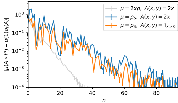
FIGURE 7. In orange and blue, for the parameters of the Lozi map a = 1.8 and b = 0.35 , |\rho_S(A \circ f^n) - \rho_S(1)\rho(A)| is plotted for varying n and two different observables A , where \rho_S = \rho(\cdot | 0) . The measure was sampled using 100 time series of 10^7 iterates of the segment dynamics f , implemented in high-precision (196-bit) validated interval arithmetic. Details of the algorithm are given in Appendix A. Two forms of error are plotted: with error bars, 99% confidence intervals for the sampling error, and with block error (not visible), the error arising from the interval arithmetic. In grey, decay of autocorrelations for a smooth observable A(x) = 2x against the SRB measure, using 100 time series of 10^8 iterates of the full dynamics f .
