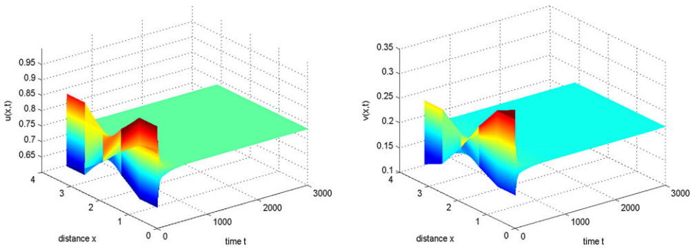
Figure 5. Taking d_2 = 0.024 , \tau = 1.95 < \tau^{(0,0)} , then E_* is stable. The initial conditions are u_0(x) = 0.76 + 0.1 \cos x and v_0(x) = 0.24 + 0.1 \cos x .
