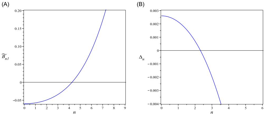
Figure 8. Taking (a, p, q, d_1, d_2, \ell) = (1, 1, 0.1, 0.01, 0.1, 4) , then (A) and (B) denote the graphs of \tilde{B}_{n1} and \Delta_n = \tilde{B}_{n1}^2 - 4A_{n1}C_{n1} , respectively. Then we obtain S = \{1, 2\} .
