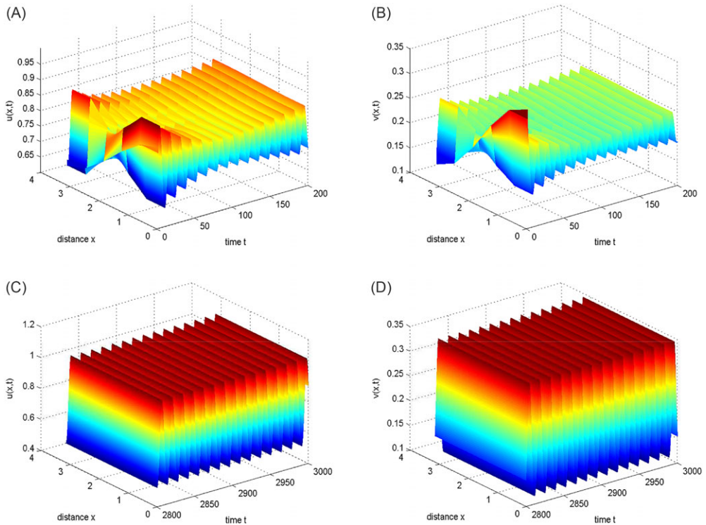
Figure 6. Taking d_2 = 0.024, \tau = 2.1 > \tau^{(0,0)} , then stable spatially homogeneous periodic solutions appear. The initial conditions are u_0(x) = 0.76 + 0.1 \cos x and v_0(x) = 0.24 + 0.1 \cos x .
