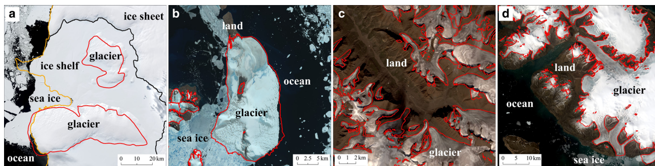
Figure 3. Examples of terminus characteristics of glaciers in the study areas. The red glacier boundaries are from RGI 6.0, with Landsat OLI scenes in (a) West Antarctica (WA) (72.8°S, 90.4°W), (b) AP (64.5°S, 57.2°W), (c) central west (CW) of Greenland (69.9°N, 53.6°W) and (d) northwest (NW) of Greenland (76.8°N, 69.3°W). The orange and black lines in (a) represent the coastlines and grounding lines, respectively.
