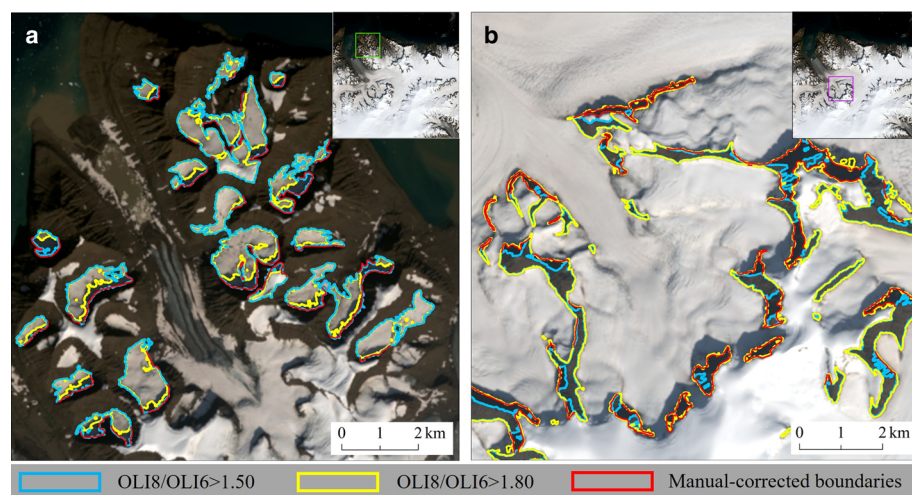
Figure 4. Shaded ice requires different thresholds for the OLI8/OLI6 ratio in dark and bright zones. The glacier scene is located in CE of Greenland (70.2°N, 25.0°W). (a) A low threshold (1.50) produces better results than a high threshold (1.80) for automatic mapping of shaded ice in dark zones. (b) A high threshold leads to better results than a low threshold for automatic mapping of shaded ice in bright zones. Correct glacier boundaries were indicated manually at the difference between them (regardless of the debris-covered ice), which generally cover blue boundaries in (a) and yellow boundaries in (b), respectively.
