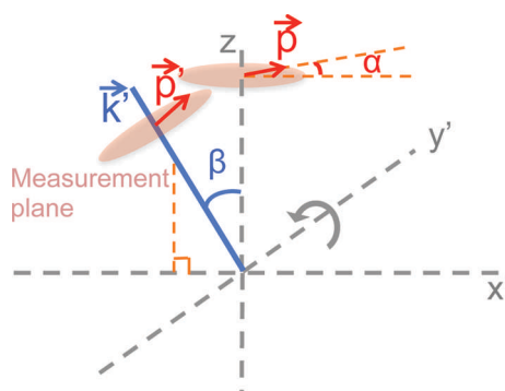
Fig. 5. Defining the polarizer extinction direction vector \vec{p}' in stage 3. Light is incident at an angle \beta from the z -axis on the x' - z plane, as described by the propagation vector \vec{k}' . Extinction occurs at an angle \alpha on the polarizer measurement plane, which is also tilted at \beta and is perpendicular to \vec{k}' . Mathematically we can define a vector \vec{p} , which is parallel to the x - y plane. We can then tilt it by \beta around the y -axis using a rotation matrix. \vec{p}' , a vector on the measurement plane at which extinction occurs, results.
