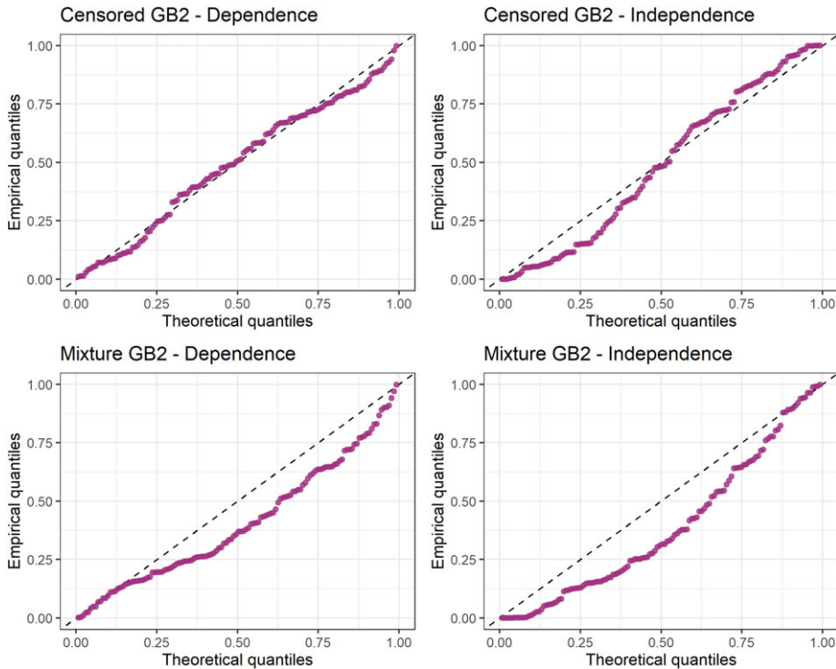
Figure 6. Q-Q plots of PIT of storm-level losses on hold-out sample for the censored (top) and two-part mixture (bottom) dependence models (left), compared to the independence case (right).
