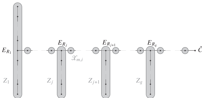
Figure 1. Resolution graph \Gamma_m for the minimal m -separating log resolution, with the irreducible components (if nonempty) of the m -contact locus \mathcal{X}_m in gray.
