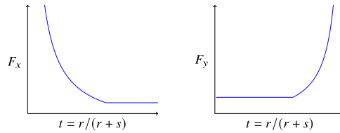
Figure 3. The graphs of F_x and F_y .
