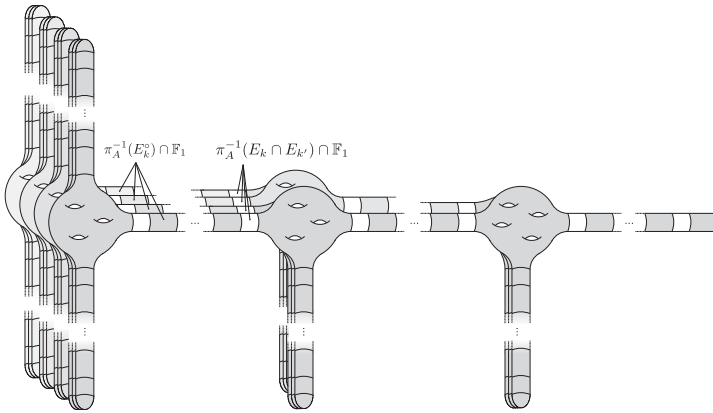
Figure 2. A'Campo decomposition of the Milnor fiber using the minimal m -separating log resolution, see [1, §2]. Note the resemblance with Figure 1.
