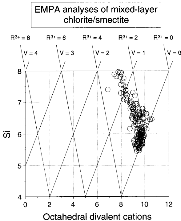
Figure 6. Plot of Si versus octahedral divalent cations exhibiting a trend given by the electron microprobe analyses of mixed-layer chlorite/smectite from the literature (see Figure 9 for references). R^{3+} = octahedral trivalent cations; V = apparent octahedral vacancies.
