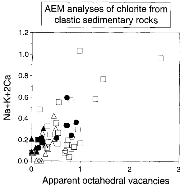
Figure 3. Relation between values of \text{Na} + \text{K} + 2\text{Ca} and apparent octahedral vacancies in published AEM analyses of chlorite in clastic sedimentary rocks ( \circ = Curtis et al 1984; \square = Curtis et al 1985; \triangle = Li et al 1994a; \bullet = Whittle 1986) and metabasites ( \blacksquare = Shau et al 1990; \blacktriangle = Shau and Peacor 1992).
