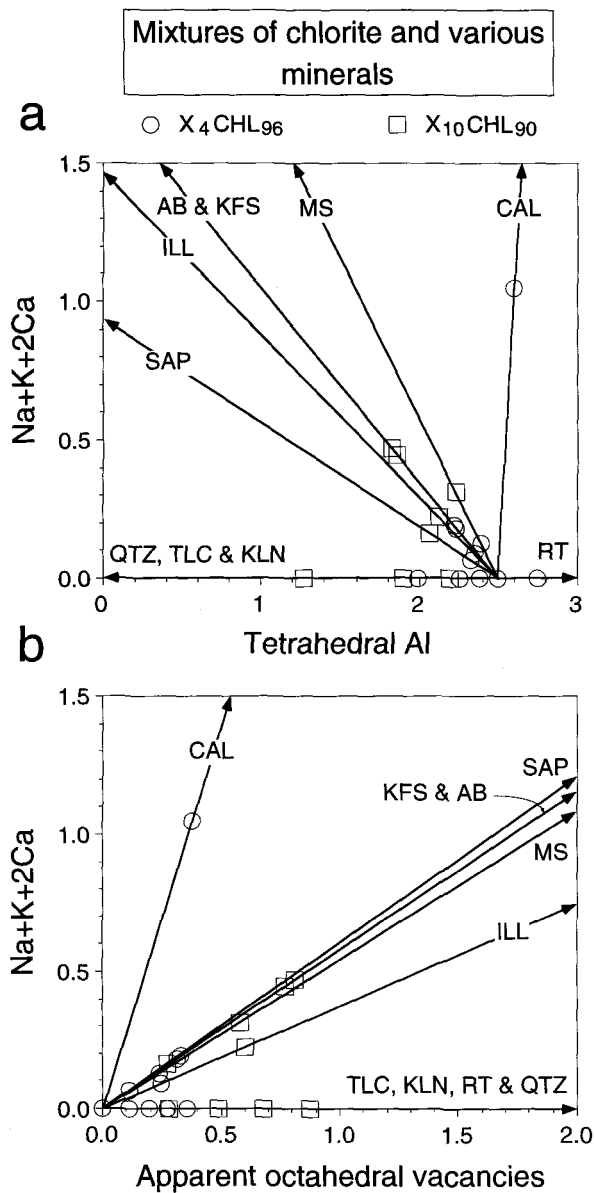
Figure 8. Diagrams showing the effects of mixing with other minerals on the values of Na + K + 2Ca, tetrahedral Al, and octahedral vacancies of chlorite. Notations and compositions for minerals are the same as those in Figure 7.
