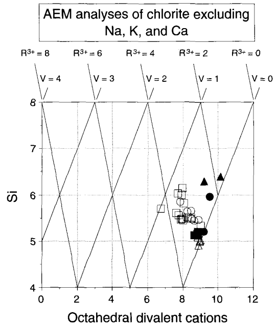
Figure 4. Plot of Si versus octahedral divalent cations (modified after Wiewióra and Weiss 1990) illustrating the extent of apparent octahedral vacancies in AEM chlorite analyses with alkali and Ca not reported ( \circ = Ahn and Peacor 1985a; \square = Jahren and Aagaard 1992; \triangle = Jiang et al 1992; \bullet = Kreuzberger and Peacor 1988; \blacksquare = Li et al 1994b; \blacktriangle = Yau et al 1988). R^{3+} = octahedral trivalent cations; V = apparent octahedral vacancies; the contours are based on 8 tetrahedral and 12 octahedral sites per \text{O}_{20}(\text{OH})_{16} .
