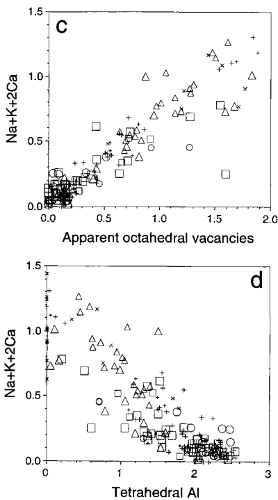
Figure 9. Diagrams showing positive and negative correlations between Na + K + 2Ca values and apparent octahedral vacancies and tetrahedral Al contents, respectively, for the
