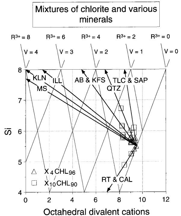
Figure 7. Plot of Si versus octahedral divalent cations displaying schematic trends of compositional deviations generated from mixtures of an assumed composition of chlorite (CHL; \text{Fe}_{5.5}\text{Mg}_4\text{Al}_{2.5}\text{Si}_{3.5}\text{Al}_{2.5}\text{O}_{20}(\text{OH})_{16} ) and other minerals. Triangles and squares represent the average compositions of 96 and 90 wt. % of the assumed chlorite plus 4 and 10 wt. % of quartz (QTZ; \text{SiO}_2 ), albite (AB; \text{NaAlSi}_3\text{O}_8 ), potassium feldspar (KFS; \text{KAlSi}_3\text{O}_8 ), calcite (CAL; \text{CaCO}_3 ), kaolinite (KLN; \text{Al}_2\text{Si}_2\text{O}_7(\text{OH})_2 ), talc (TLC; \text{Mg}_3\text{Si}_4\text{O}_{10}(\text{OH})_2 ), saponite (SAP; \text{Ca}_{0.4}\text{Na}_{0.2}\text{Mg}_6\text{Si}_7\text{AlO}_{20}(\text{OH})_4 ), muscovite (MS; \text{K}_2\text{Al}_4\text{Si}_6\text{Al}_2\text{O}_{20}(\text{OH})_4 ), illite (ILL; \text{K}_{1.4}\text{Al}_4\text{Si}_{6.6}\text{Al}_{1.4}\text{O}_{20}(\text{OH})_4 ), and rutile (RT; \text{TiO}_2 ), respectively. R^{3+} = octahedral trivalent cations; V = apparent octahedral vacancies.
