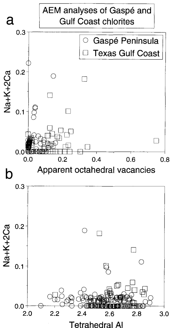
Figure 2. Correlation diagrams showing relations between Na + K + 2Ca values and apparent (a) octahedral vacancies and (b) tetrahedral Al content of chlorite in pelitic rocks from the Gaspé Peninsula and Texas Gulf Coast.
