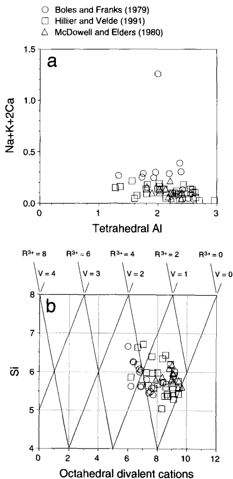
Figure 5. Diagrams displaying the relations (a) between tetrahedral Al and \text{Na} + \text{K} + 2\text{Ca} contents, and (b) among octahedral divalent cations, Si content, and apparent octahedral vacancies for published electron microprobe analyses of chlorite in clastic sedimentary rocks. R^{3+} = octahedral trivalent cations; V = apparent octahedral vacancies.
