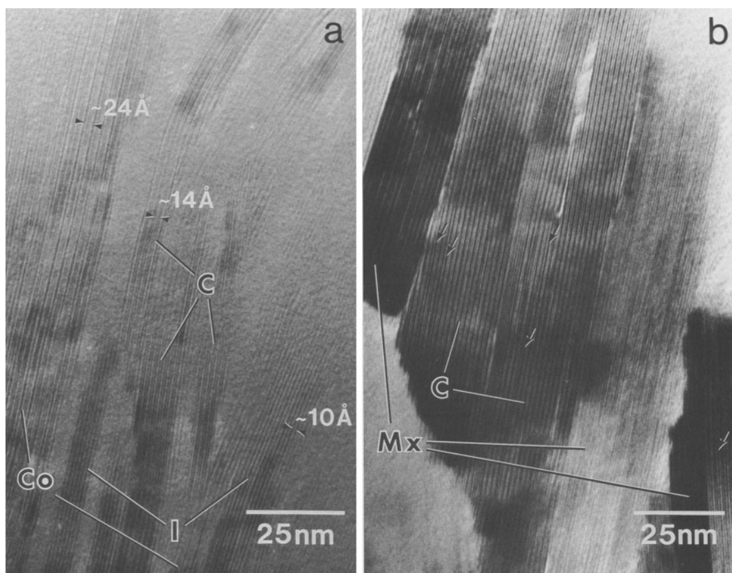
Figure 1. Transmission electron microscope images of (a) chlorite (C; d(001) \cong 14 \text{ \AA} ) coexisting with corrensite (Co; d(001) \cong 24 \text{ \AA} ) and illite (I; d(001) \cong 10 \text{ \AA} ) in sample A416 of the diagenetic zone of the Gaspé Peninsula, Quebec, and (b) aggregates of packets of chlorite (C) interstratified with local \sim 7\text{-\AA} layers (black arrows) in a shale recovered from a depth of 4741.8 m; Pleasant Bayou #1 well, Brazoria County, Texas. Mx = mixed-layer 7- \text{\AA} /14- \text{\AA} phase.
