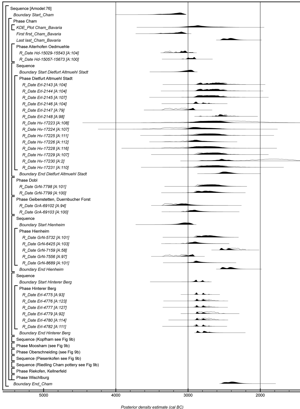
Fig. 9. (above & opposite). Probability distributions for radiocarbon measurements associated with the use of Cham material culture in Bavaria. The brackets and CQL2 key words define the model, as does the code given in Appendix S4 (plot: S. Griffiths)
