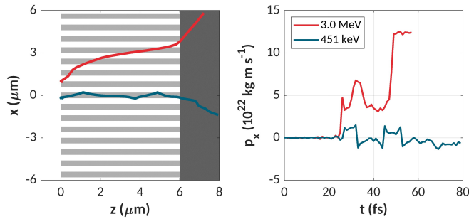
Figure 8: The transverse momenta of two example fast electrons as they traverse the wire region. The blue trajectory and plot is for an electron with a final energy close to the ponderomotive temperature, and the red trajectory and plot is for one of the highest energy MeV electrons.
