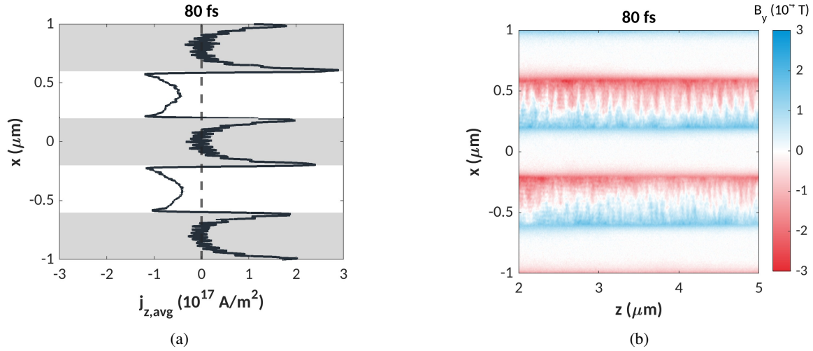
Figure 7: (a) Current density j_z averaged between z = 2 - 5 \mu\text{m} . Shaded regions indicate the wire positions and the white regions indicate vacuum. (b) Corresponding B_y fields (orthogonal to the simulation plane) within the same region.
