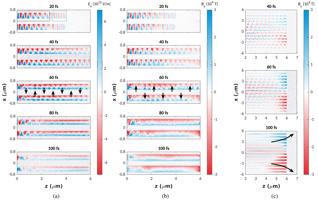
Figure 6: E_x (a) and B_y (b) field components around the central wire for the p -polarised PIC simulation. Black arrows indicate the direction the fields will act on an electron propagating in z . The B_y field is shown in (c) across the whole target. The black arrows here indicate the direction of deflection of an electron propagating in the +z direction.
