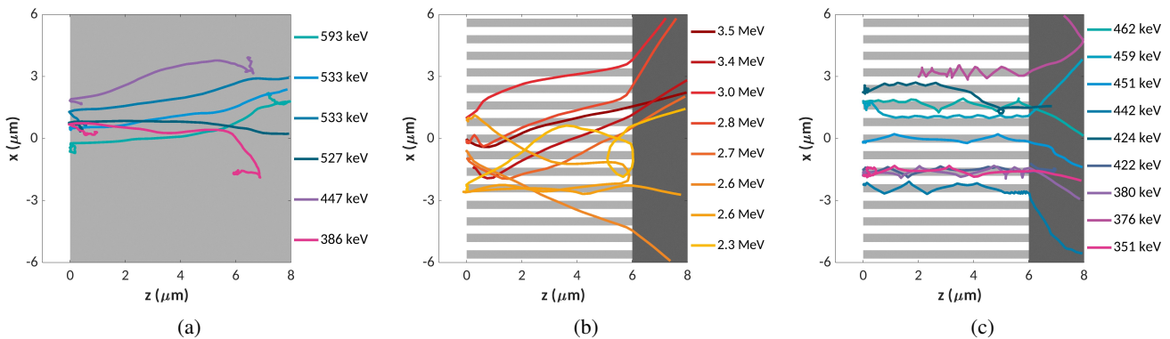
Figure 5: Electron trajectories from a random subset of hot electrons from the p -polarised laser interactions. The electron path is plotted across 120 fs, and is labelled according to the maximum energy reached during the simulation. Figures (a) and (b) show example trajectories of the highest energy electrons for the planar and nanowires respectively, and (c) shows example trajectories of lower energy electrons with E_{max} \sim 400 keV from the nanowire interaction.
