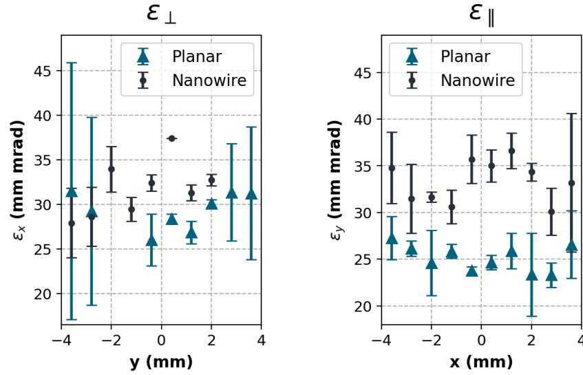
Figure 3: Experimental estimate of the transverse emittance in (a) x , perpendicular to the laser \mathbf{E} -field, and (b) y , parallel to the \mathbf{E} -field. Error bars are taken from the uncertainty introduced from the background correction applied.
