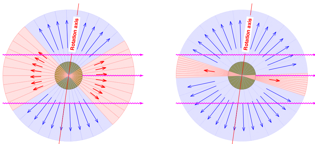
Figure 4. Left panel: Sketch of the geometry of the two-zone model for Sk 190. From the observer located to the right, nearly the whole stellar surface is seen through the slow wind of the equatorial zone. Therefore, the absorption part of the P-Cygni profile is narrow, according to a maximum blue-shift of -v_{\infty} . Those rays which are missing the stellar disk, however, collect emission from the fast polar wind, including matter in the back hemisphere that shows large red-shift leading to the broad emission part. Right panel: Sketch of the geometry of the two-zone model for \zeta Oph. As seen from the observer located to the right, the disk-like region obscures roughly half of the stellar surface, causing an extra absorption at about zero Doppler shift.
