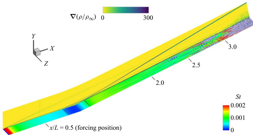
Figure 12. Instantaneous flow for case A1.5. Stanton number is shown together with isolines of zero skin friction coefficient. Density gradient at z/L = 0 is shown to indicate the SBLI. The Q -criteria is used to visualise the transitional and turbulent flow.
