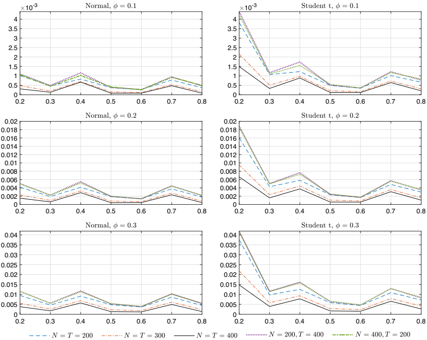
FIGURE 2. \text{Bias}_\beta^2 .
