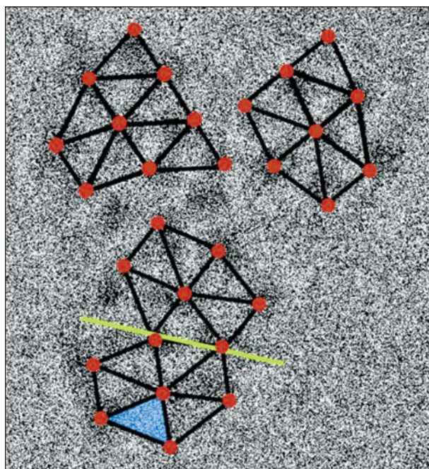
Relative position of molecules derived from the x-ray diffraction crystal structure (red circles) overlaid on the transmission electron microscope image. Credit: Nature Chemistry .
