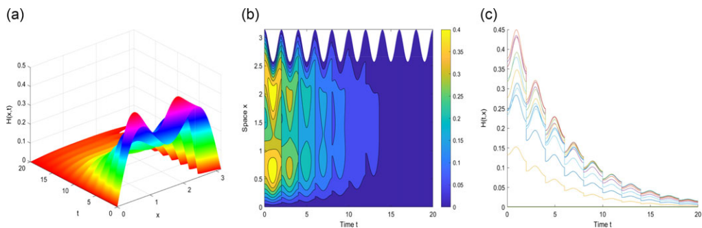
Figure 2. \rho_1(t) = e^{-0.1(1-\cos(\pi t))} , n_1 = 8 and n_2 = 10 . The domain is periodically evolving with \rho_1 and R_0^2 < 1 . Graphs (a)–(c) show that the population H(t, x) decays to 0. Graphs (b) and (c) are the cross-sectional view and projection of H on the t - H plane, respectively. The colour bar in graph (b) shows the density of H(t, x) .
