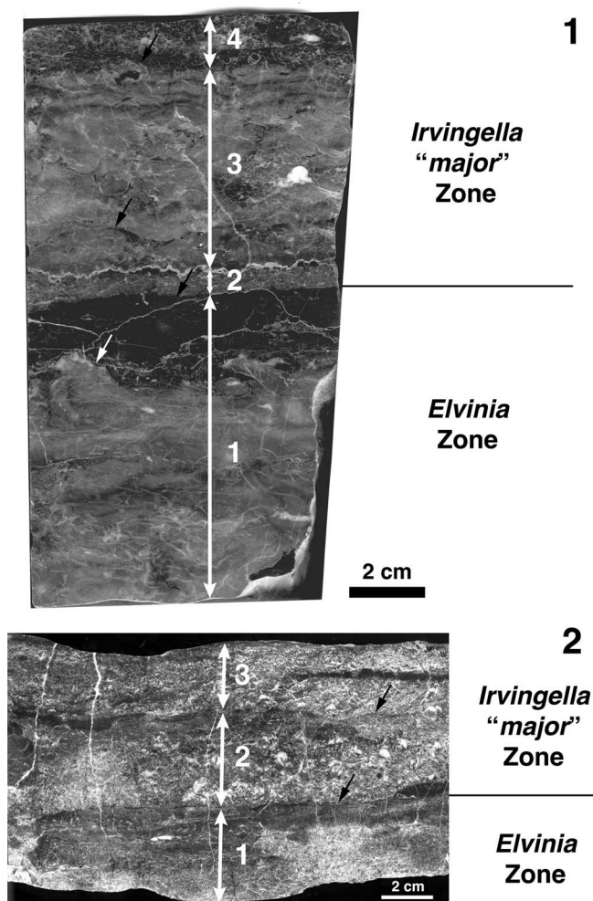
Figure 9. Condensed shell bed (including the Irvingella “major” coquina that marks the base of the Sunwaptan Stage and the onset of faunal change) at the top of the Barton Canyon Limestone Member. Short white and black arrows show internal hardgrounds. (1) Sample CHC-1-0. Each of the four layers was sampled separately for carbon isotopes and trilobites. The upper half of the slab is the Irvingella “major” Zone and is divisible into three layers (2–4). Layer 2 is bioclastic grainstone; layer 3 is bioclastic pack- and rudstone; layer 4 is bioclastic grain- to rudstone. Layer 1 yields a trilobite fauna of the Elvinia Zone and includes light gray lime mudstone to wackestone and black lime mudstone. Trilobite abundance data for layers 1, 3, and 4 are shown in Figure 14. (2) Sample STR 11.9–12.1. Three layers of bioclastic grain- to rudstone were sampled separately for trilobites, each of which is separated by a well-defined, irregular hardground (short black arrows); layer 1 contains the of the Elvinia Zone; layers 2 and 3 comprise the Irvingella “major” coquina. Trilobite abundance data for each of the layers are shown in Figure 14.
