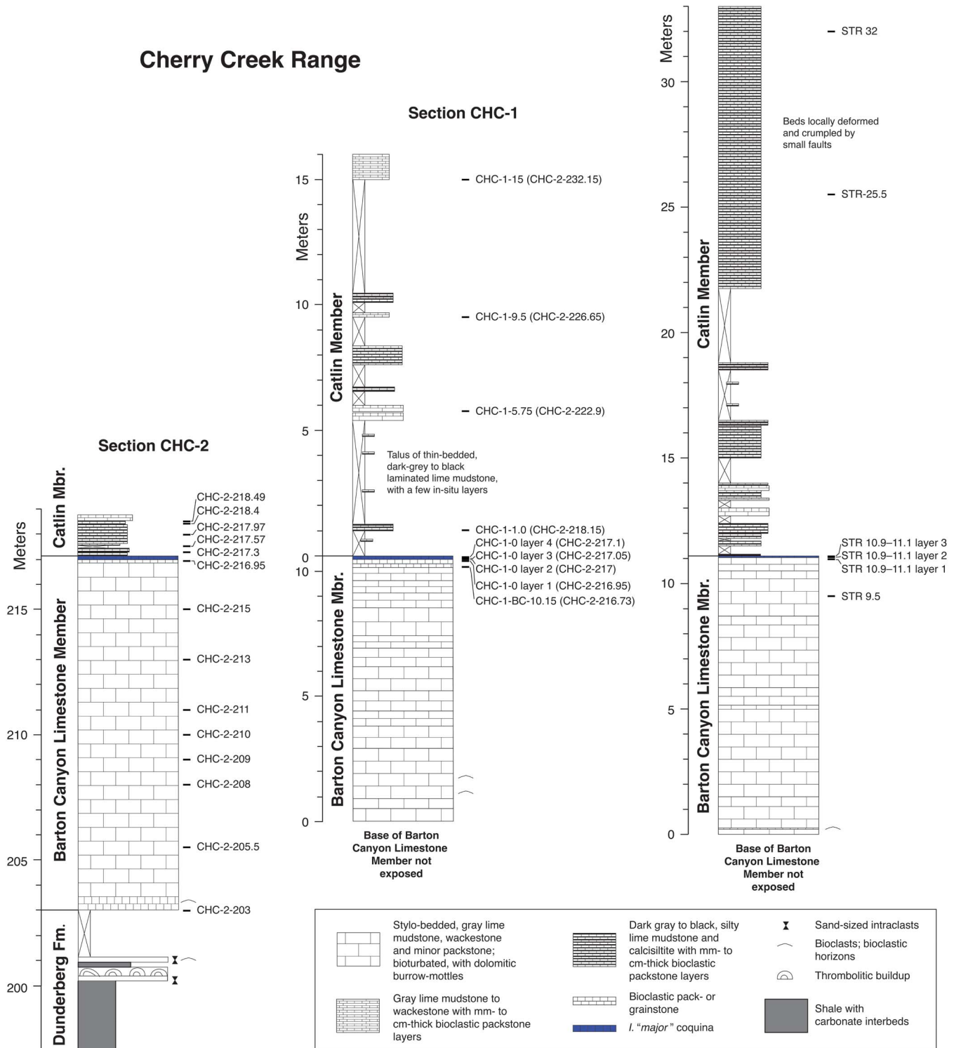
Figure 3. Stratigraphic columns for measured sections at Barton Canyon, Cherry Creek Range (CHC-1 and CHC-2; Fig. 1.2) and on the Steptoe Ranch, North Egan Range (STR; Fig. 1.1). The sections are aligned using the top of the Irvingella "major" coquina at the top of the Barton Canyon Limestone Member of the Windfall Formation as a datum. Sample horizons are in meters. Sample meterages in parentheses for section CHC-1 are equivalent levels in the composite section for Barton Canyon Limestone Member used to plot carbon isotope and genus range data (Figs. 17, 19). Positions in the composite section were calculated using the top of the Barton Canyon Limestone Member as a datum, and projected onto CHC-2, which is the most completely sampled of the two sections.
