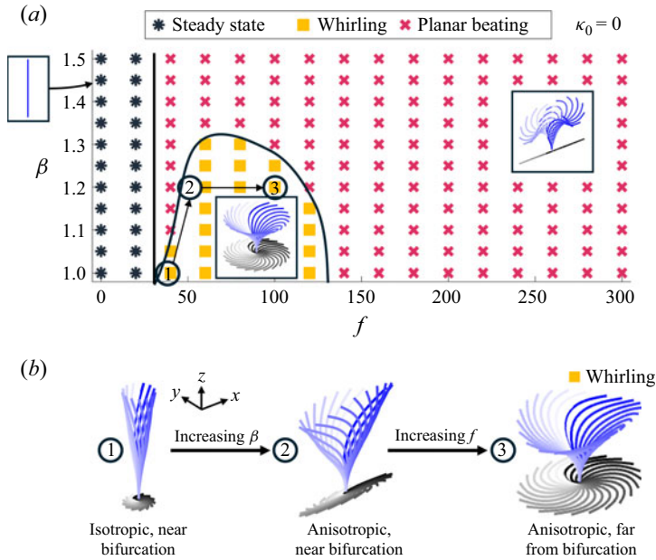
Figure 6. (a) Results of numerical simulations of an anisotropic filament with no intrinsic curvature ( \kappa_0 = 0 , \beta \geq 1 ). The black lines are drawn to indicate the approximate boundaries of the solution regions. (b) Snapshots of filaments over one period undergoing whirling dynamics in the isotropic case, close to the bifurcation ( \beta = 1 , f = 36 ), an anisotropic case near the bifurcation ( \beta = 1.2 , f = 46 ) and an anisotropic case further from the bifurcation ( \beta = 1.2 , f = 100 ). The three dynamics are indicated on the phase diagram in (a) using numbered circles.
