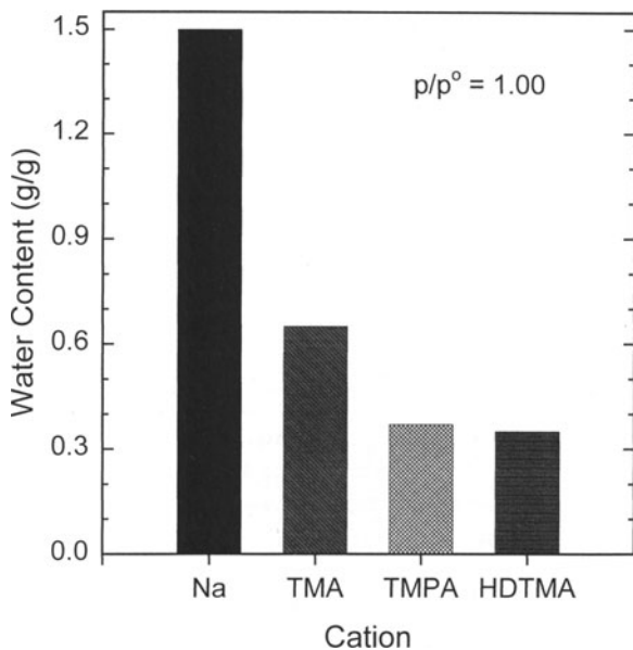
Figure 1. Equilibrium water content ( m_w/m_c ) at 100% relative humidity ( p/p^o = 1.00 ) of SWa-1 saturated with Na or with one of three organo-cations.
