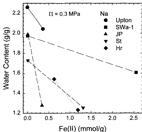
Figure 3. Effect of Fe oxidation state on equilibrium water content of five Na-saturated smectites equilibrated at \Pi = 0.3 MPa.
