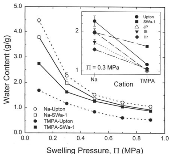
Figure 2. Effect of swelling pressure ( \Pi ) on equilibrium water content ( m_w/m_c ) of unaltered (oxidized) SWa-1 and Upton saturated with Na or TMPA. Inset compares water contents of Na- and TMPA-saturated smectites JP, St, or Hr with SWa-1 and Upton at \Pi = 0.3 MPa.
