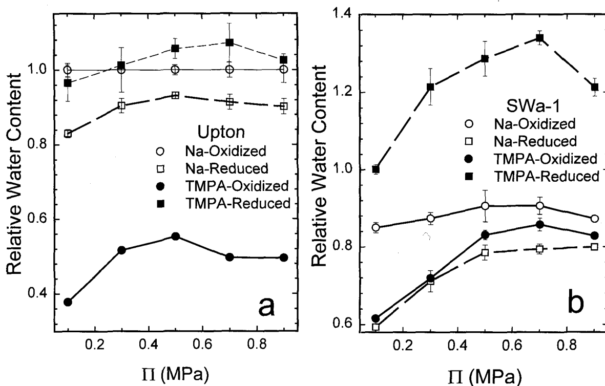
Figure 5. Comparisons of the effects of interlayer cation (Na or TMPA) and Fe oxidation state on the relation between equilibrium water content ( m_w/m_c ) and swelling pressure ( \Pi ) for (a) Upton, and (b) SWa-1. All H_2O -content values are relative to oxidized Na-saturated Upton at the corresponding value of \Pi .
