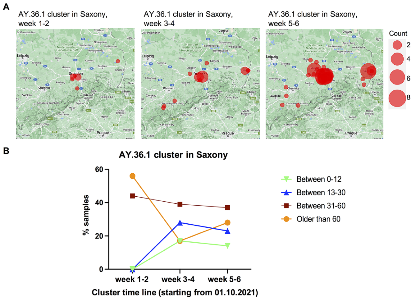
Figure 5. Dynamic changes of geographic distribution and age distribution of detected new samples in the AY.36.1 cluster in every 2 weeks along with the cluster timeline. (a) The geographic distribution of detected new samples in the AY.36.1 cluster in Saxony, Germany in every 2 weeks along with the cluster timeline is displayed based on documented postcodes. (b) The age distribution of detected new samples in the AY.36.1 cluster in every 2 weeks is displayed.
