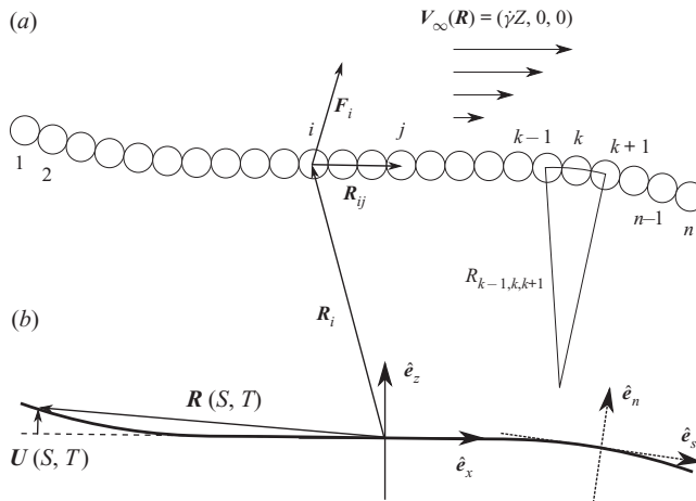
Figure 1. Models of a fibre in shear flow and the notation. (a) The bead model. (b) The elastica model.
