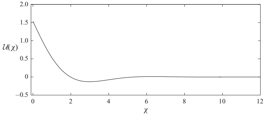
Figure 6. Similarity solution from the elastica model (4.7)–(4.8a–c), valid at early times, for a fibre initially aligned with the flow.
