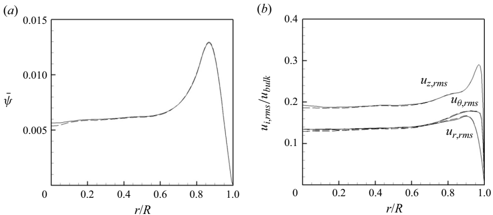
Figure 5. Profiles of the (a) mean bubble volume fraction and (b) r.m.s. velocity fluctuations for different axial domain sizes (case ML): —, L_z = 3D ; - - -, L_z = 6D .
