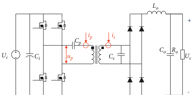
FIGURE 10: The diagram of the setups for measuring.
