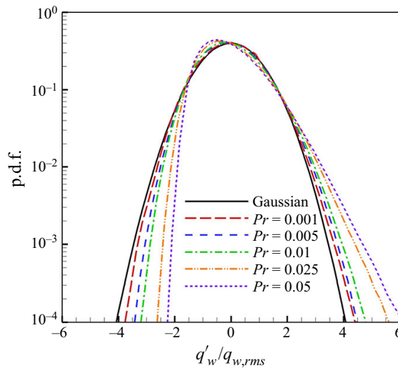
Figure 24. Probability density function (p.d.f.) of surface heat flux for low Pr obtained using DNS.
