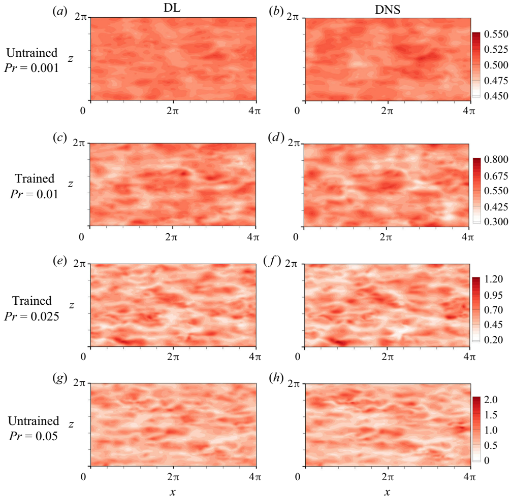
Figure 25. Instantaneous surface heat flux for low Pr obtained from wall-shear stresses using cGAN.
