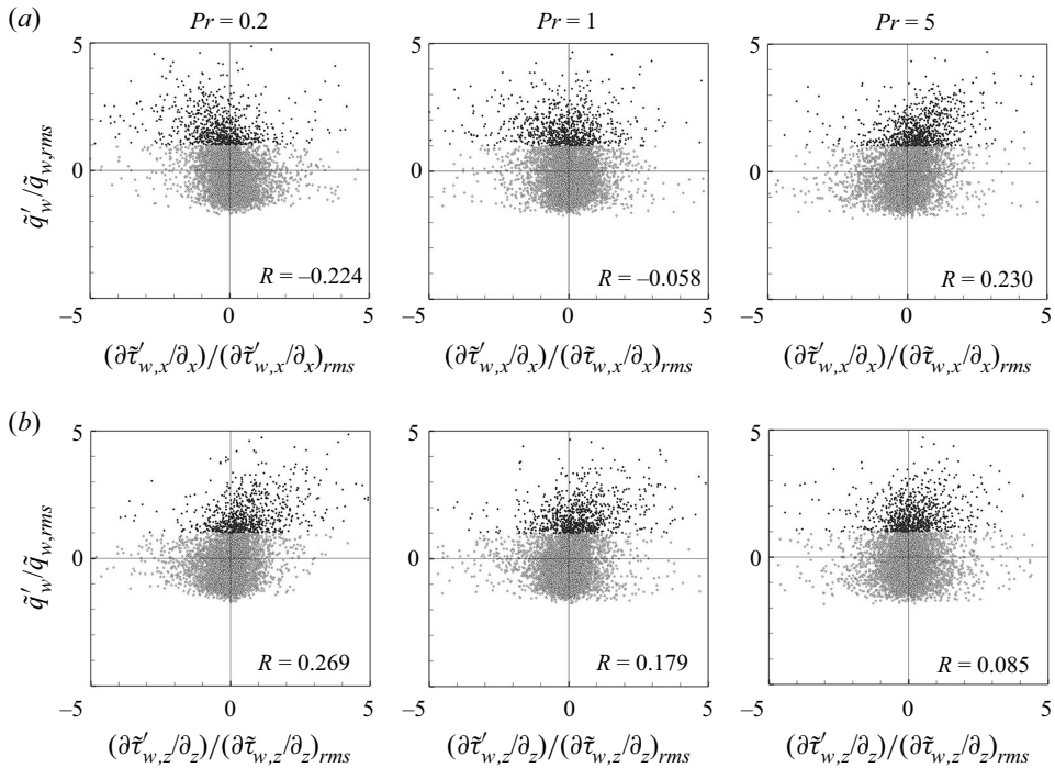
Figure 16. Scatterplots between surface heat flux with Pr and gradient of (a) streamwise wall-shear stress \partial \tilde{\tau}'_{w,x} / \partial x and (b) spanwise wall-shear stress \partial \tilde{\tau}'_{w,z} / \partial z . High heat flux data ( \tilde{q}'_w > \tilde{q}'_{w,rms} ) are marked with darker points to highlight the correlation.
