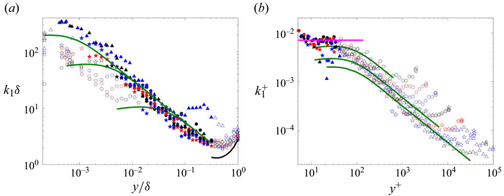
Figure 3. Wall-normal dependence of the peak associated with LSM in (a) outer scaling and (b) inner scaling. The green lines in (a) indicate \mu_1\delta/y for Re_\tau = 2000 , 20 400 and 1 00 000, and the black line shows the peak of f_{HT} (see (2.3)). In (b), the green lines show \mu_1/y^+ for Re_\tau = 2000 , 20 400 and 1 00 000, and the pink line marks \mu_3/y^+ (see (2.12)). The symbols and colours are given in table 1, with the filled symbols used to indicate when y^+ > 30 and y/\delta \leq 0.3 in (a), and when y^+ \leq 30 in (b).
