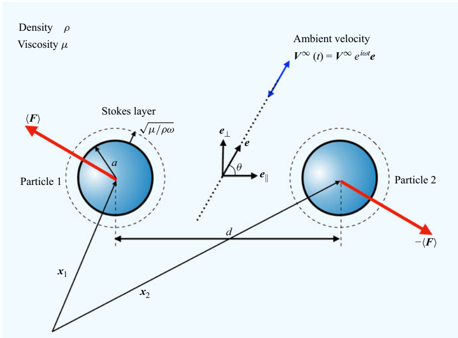
Figure 1. Sketch showing two identical particles suspended in a uniform ambient oscillatory flow \mathbf{V}^{\infty}(t) . Hydrodynamic interactions between the particles, due to advective nonlinearities, drive secondary time-averaged forces and drift velocities of the particles.
