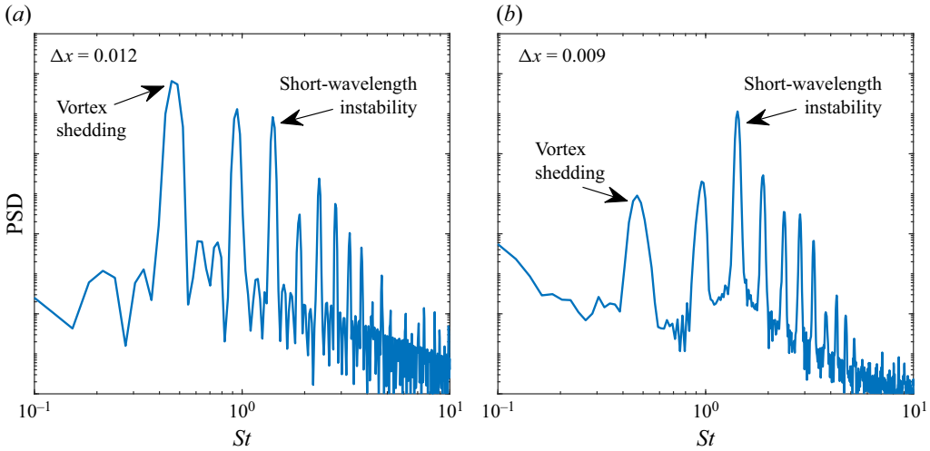
Figure 2. PSD for Re = 500 , \alpha = 25^\circ and \lambda = 3 with grid resolutions of (a) \Delta x/D = 0.012 (case B1) and (b) \Delta x/D = 0.009 (case B2). The Nyquist frequencies are St = 500 and St = 667 , respectively. Note that y-axes are logarithmic. Frequency bin size differs between the two plots.
