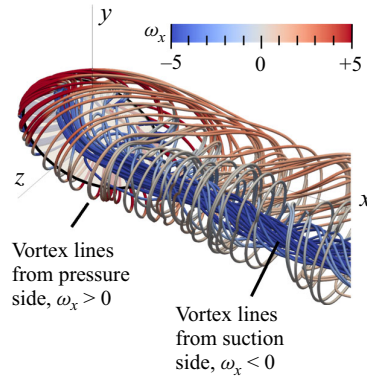
Figure 10. Visualisations of vortex lines for steady flow over the disk at Re = 500 , \alpha = 25^\circ and \lambda = 1.5 . The free stream velocity is in the positive x -direction (approximately top left to bottom right). Vortex lines extend from the suction side of the disk, seeded in a ring parallel to the disk with a normal distance 0.1D and diameter 0.5D , and are coloured by streamwise vorticity, \omega_x . The maximum length of vortex lines is 40D . Vortex lines eventually loop back towards the disk.
