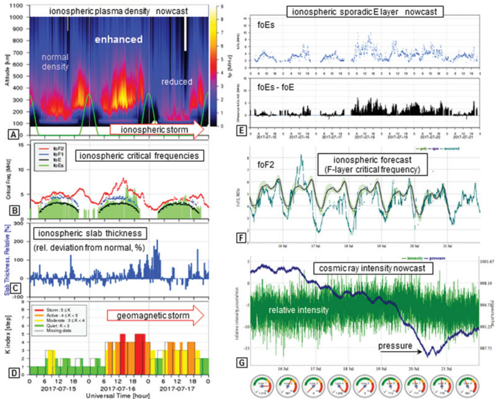
Figure 1. Space weather monitoring services ( http://ionosphere.meteo.be ): (A) ionospheric plasma density (plotted as plasma frequency) nowcast, (B) ionospheric critical frequencies, (C) ionospheric slab thickness, (D) geomagnetic activity nowcast, (E) ionospheric sporadic E-layer activity nowcast, (F) ionospheric forecast (climatological), and (G) cosmic ray intensity nowcast.
