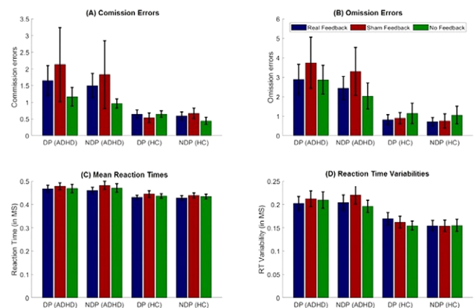
Figure 1. CPT results. DP=distractor-phases, NDP=non-distractor-phases
