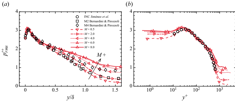
Figure 4. Intensities of pressure fluctuations p'_{rms} shown in (a) the outer scale and (b) the inner scale. The circles indicate the reference data of an incompressible TBL with Re_\tau = 690 from Jiménez et al. (2010). The squares and diamonds denote M = 2 and 4 TBLs with Re_\tau = 508 and 506 , respectively, from Bernardini & Pirozzoli (2011).
