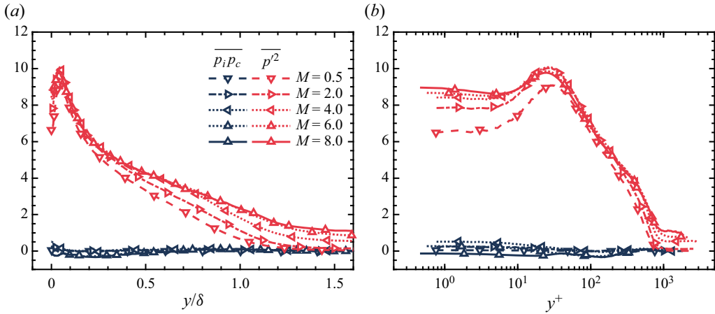
Figure 11. Comparisons of intensities of pressure fluctuations \overline{p^2} and interactions between pressure components \overline{p_i p_c} in (a) the outer scale and (b) the inner scale.
