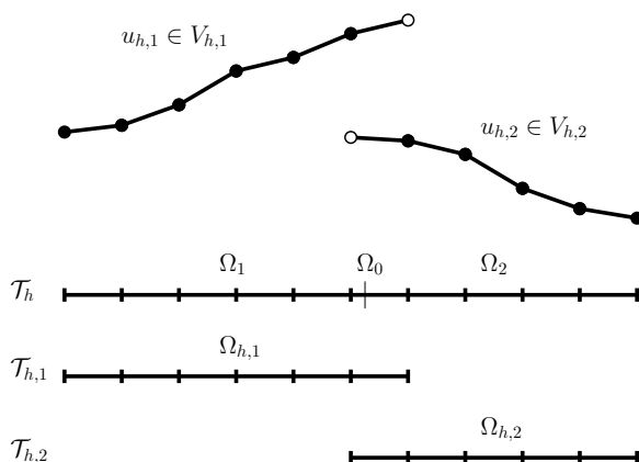
Figure 2.3. An illustration in one space dimension of how a solution u_h \in W_h from the cut finite element method (2.40) might look. Note that u_h = (u_{h,1}, u_{h,2}) , where u_{h,i} \in V_{h,i} for i = 1, 2 , with V_{h,i} here consisting of continuous piecewise linear finite elements.
