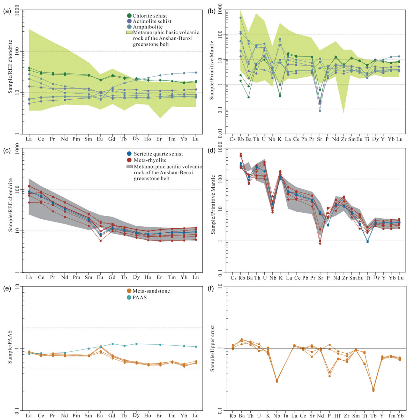
Figure 7. Chondrite normalized REE (a,c: normalized values after Boynton 1984), and primitive mantle normalized spider diagrams (b,d: normalized values after Sun and McDonough 1989) of sericite quartz schist, meta-rhyolite, chlorite schist, actinolite schist and amphibolite in the Anshan-Benxi area; PAAS-normalized REE patterns (e: normalized value after McLennan, 1989) and upper crust-normalized trace element spider diagram (f: normalized value after Taylor and McLennan, 1985) of meta-sandstones in the Anshan-Benxi area. (a,b) Metamorphic basic volcanic rock; (c,d) Metamorphic acidic volcanic rock; (e,f) Meta-sandstone.
