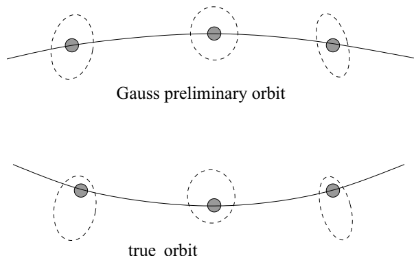
Figure 1. Qualitative sketch in which the orbit given by Gauss's method (preliminary orbit plus differential corrections) presents a curvature that is not reliable at all.
