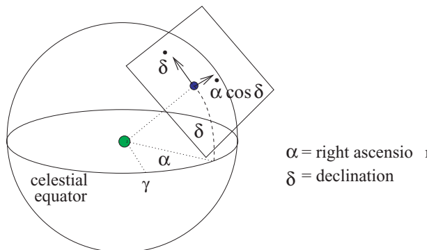
Figure 2. The celestial sphere and the components of an attributable.
