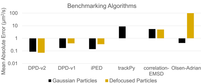
Figure 14. Mean absolute errors ( \mu\text{m}^2\text{s}^{-1} ) of various methods on Gaussian and defocused datasets. The experiments were done with 20 frames.
