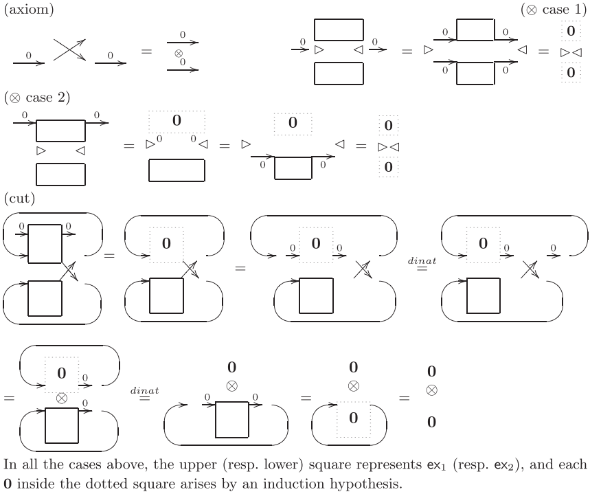
Figure 8. Pictorial Proof of Lemma 4.14.
