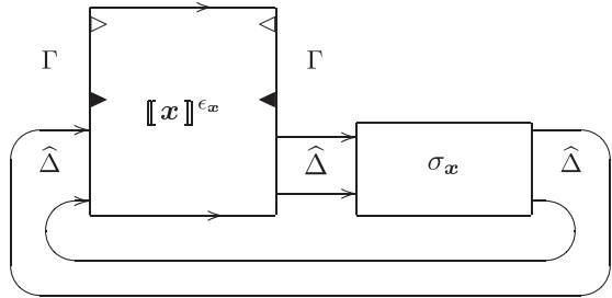
Figure 6. Execution formula Ex(\sigma, \mathbf{x}) , where \blacktriangleright (resp. \blacktriangleleft ) denotes \triangleright^0 (resp. \triangleleft^0 ).
