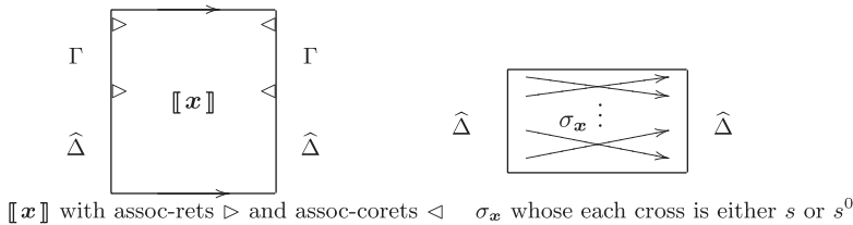
Figure 1. (\llbracket \mathbf{x} \rrbracket, \sigma_x) of Definition 4.4 and assoc-rets and assoc-corets of Definition 4.4.
