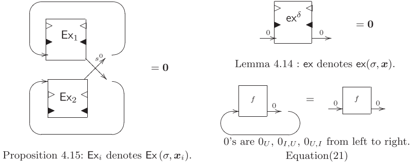
Figure 7. Proposition 4.15 and Lemma 4.14 and Equation (21) pictorially, where \blacktriangleright and \blacktriangleleft denote respectively \triangleright^0 and \triangleleft^0 .
