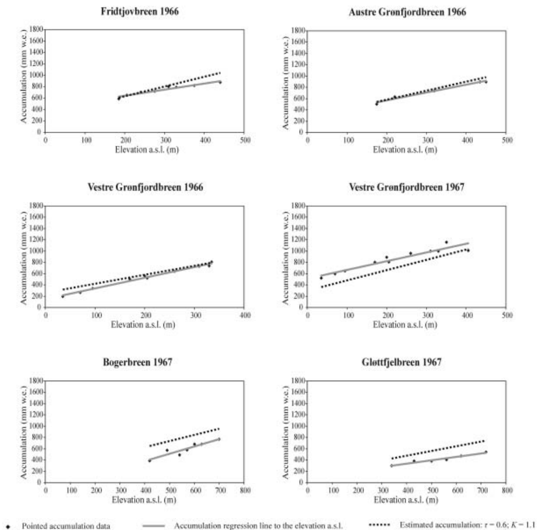
Fig. 3. Observed and modeled values of accumulation on Fridtjovbreen, austre Grønfjordbreen, vestre Grønfjordbreen, Bogerbreen and Gløttfjellbreen in the years 1966–67.
