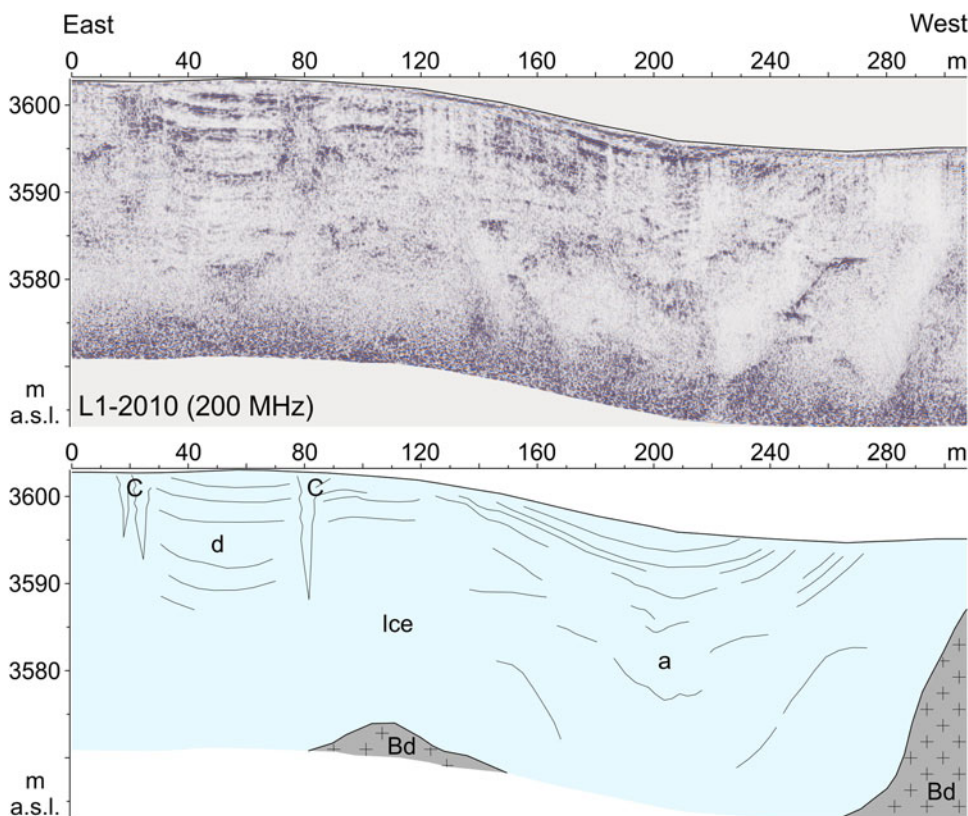
Fig. 13. GPR scanline L1-2010 collected with a 200 MHz transducer: processed data (top) and interpretation (bottom). The ice layer appears to be quite reflective, and some curved reflectors (marked ‘a’ and ‘d’), as well as some crevasses (marked ‘C’) with their typical diffraction patterns, are clearly imaged. The curved reflectors correspond to the zones of minima in the V_p velocity maps. Bd, bedrock; C, crevasse. See text for description.
