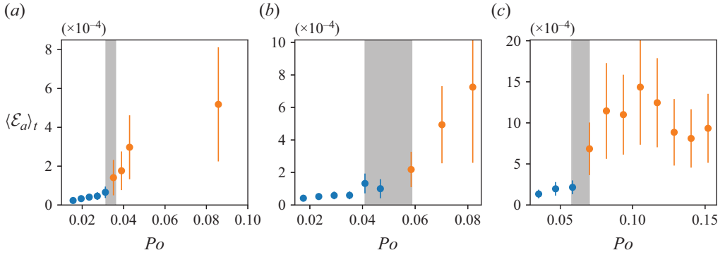
Figure 7. Time-averaged anti-symmetric kinetic energy \langle \mathcal{E}_a \rangle_t measured on the principal axes of the ellipsoid as functions of Po for three investigated Ekman numbers. Stable points are displayed in blue, unstable points in orange, and the error bars are representative of the standard deviation over the entire time series. The grey shaded area represents a region of uncertainty for the onset of instabilities. Here, (a) E = 2.1 \times 10^{-5} , (b) E = 3.1 \times 10^{-5} , and (c) E = 6.3 \times 10^{-5} .
