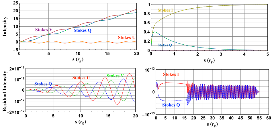
Figure 2. Polarised GRRT tests I. Left column: pure polarised emission in Stokes ( Q, U, V ), I = 0 (top panel) and residuals compared to analytic solution (bottom panel). Right column: pure emission and absorption in Stokes ( I, Q ), U = V = 0 (top panel) and residuals compared to analytic solution (bottom panel). Analytic solutions are plotted as dashed lines in upper panels.
