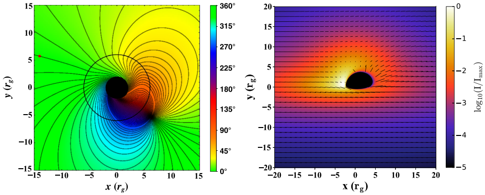
Figure 3. Polarised GRRT tests II. Left panel: EVPA contour map ( \tilde{\chi} \equiv \chi + \pi ) of a Keplerian accretion disk around a Schwarzschild BH as viewed at 30^\circ . The black ring denotes the innermost stable circular orbit (ISCO), wherein the disk material is in free-fall. The red dot corresponds to the \tilde{\chi} = 0^\circ contour. Right panel: Novikov-Thorne accretion disk with electron scattering atmosphere around an extremal Kerr black hole. Colour denotes the total intensity integrated over the range 0.1–10 keV, \dot{M} = 0.1 M_{\text{Edd}} , M = 10 M_\odot and viewed at 75^\circ . Orientation of black ticks indicates the polarisation direction, and the length of each tick denotes the polarisation degree ( \sim 5\% at bottom of panel). Significant depolarisation and enhancement can be seen.
