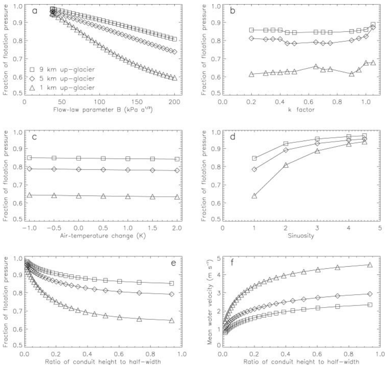
Fig. 5. (a–e) The influence of various parameters on the water pressure at three distances from the ice margin in a selected subglacial channel. The legend in (a) is valid for all plots. See text for a detailed explanation of the plots. (f) Calculated mean water speed in the subglacial channel as a function of channel geometry.
