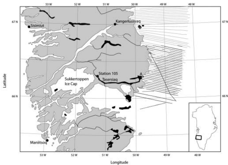
Fig. 1. Overview of the region studied. The grey lines on the ice sheet show the extent of the airborne survey carried out in 2003, and the black lines signify which part was utilized for this work. The point marked A shows the position of a weather station on the ice sheet and also marks the outlet of the hypothetical drainage channel used for calculations of basal water pressure.
