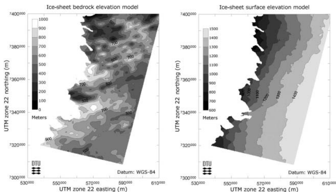
Fig. 2. Contour maps of the bed and surface elevation models. See text for details.
