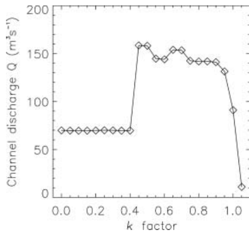
Fig. 3. The channel meltwater discharge Q as a function of the k factor in Equation (1). The k factor causes changes in the drainage basin extent, and thus indirectly in the meltwater discharge Q .
