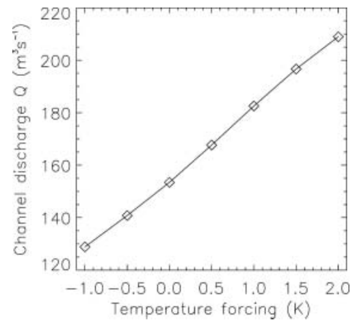
Fig. 4. The channel meltwater discharge for the basin corresponding to a k factor of 0.7 as a function of the 3 m level air-temperature forcing off the ice sheet.
