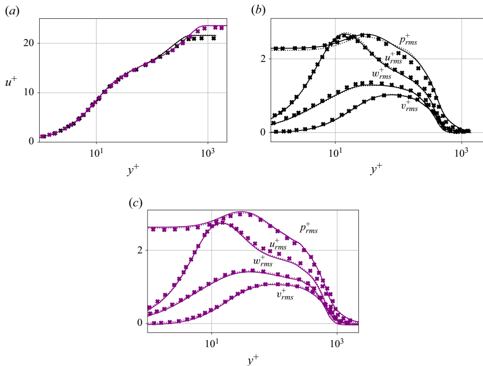
Figure 3. A comparison of DNS of the current method with that of Biau (2023): (a) mean streamwise velocity u^+ ; (b) r.m.s. velocities and pressures at Re_\theta = 1000 ; (c) r.m.s. velocities and pressures at Re_\theta = 2000 . Data from Biau (2023) are shown with markers ( \times Re_\theta = 1000 ; \times Re_\theta = 2000 ), from the present DNS using f_{DNS} with solid lines ( — Re_\theta = 1000 ; — Re_\theta = 2000 ) and from the implementation of Biau's method in Xcompact3d with dotted lines ( ..... Re_\theta = 1000 ; ..... Re_\theta = 2000 ).
