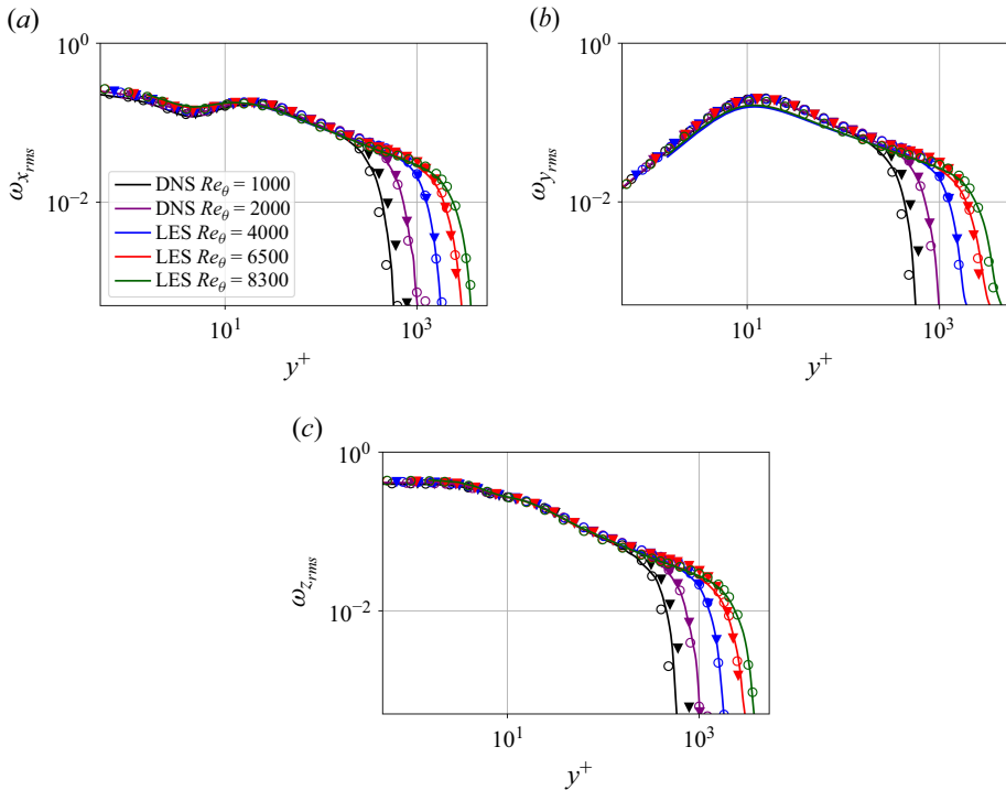
Figure 8. Profiles of the r.m.s. vorticity components (a) \omega_{x,rms} ; (b) \omega_{y,rms} ; and (c) \omega_{z,rms} , for Re_\theta = 1000 to 8300 . Reference data are shown with markers: ( \circ ) for both the DNS of Schlatter & Örlü (2010) and the LES of Eitel-Amor et al. (2014); ( \blacktriangledown ) for the DNS of Sillero et al. (2013). Results with the present method are shown with solid lines.
