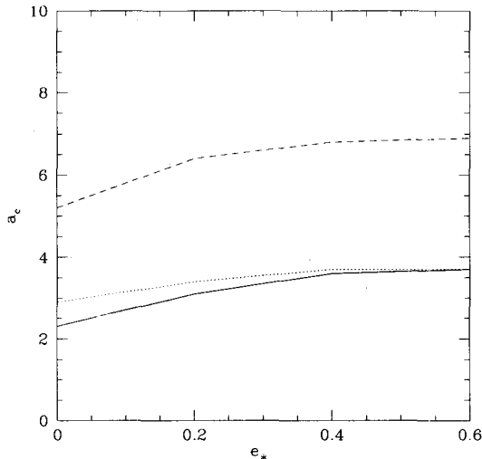
Fig. 2. The same as in Fig.1 except that the mass ratio of the binary system \mu = 0.5 .
