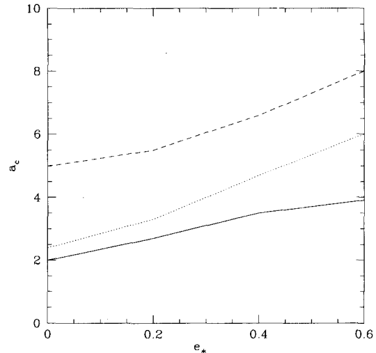
Fig. 1. The critical semi major axis as a function of eccentricity when the mass ratio of the binary system \mu = 0.1 . The solid line represents the result for models with brown dwarfs treated as massless test particles which initially move on circular orbits. These models are analogous to those obtained by Holman & Wiegert (1999). The dotted line represents the results for models in which brown dwarfs are assigned the finite mass \mu_b = 0.05 . The brown dwarfs are assumed to have circular orbits about the center of mass of the binary system initially. The dashed line represents the results of models in which brown dwarfs have mass \mu_b = 0.05 and initial eccentricity e_b = 0.4 .
