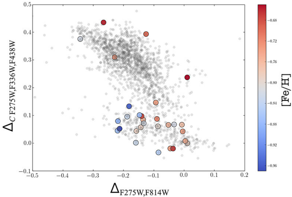
Figure 4. Chromosome map of red giant branch stars in the GC 47 Tucanae, with super-imposed stars with available FLAMES-UVES spectra. The color of the spectroscopic targets is indicative of the inferred iron chemical abundance, as indicated by the column bar on the right (Marino et al. 2023a).
