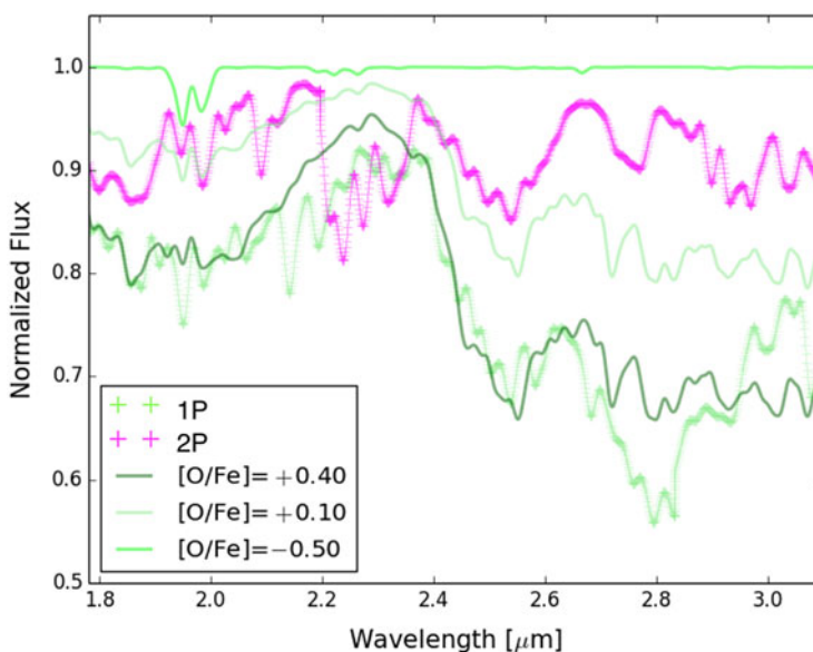
Figure 10. Two observed NIRSpectra of 47 Tucanae M dwarfs. Green and magenta crosses represent a 1P and 2P M dwarf, respectively. Super-imposed to the observed spectra are three spectra simulated at [O/Fe] = -0.50, +0.10, +0.40 dex.
