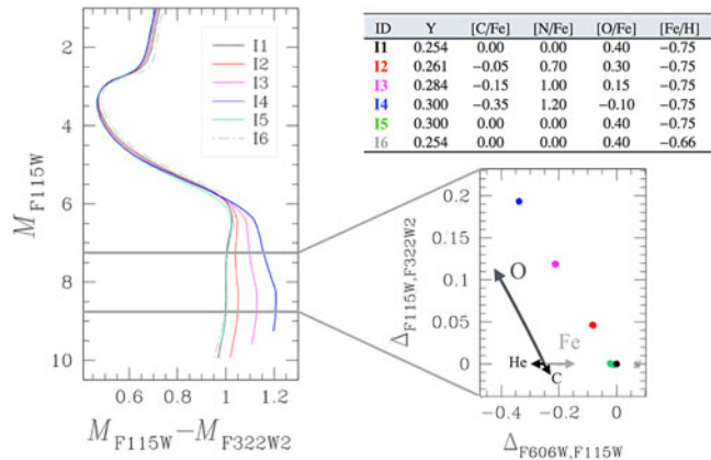
Figure 6. Isochrones in the M_{F115W} vs. M_{F115W} - M_{F322W2} plane, constructed by assuming the different chemical abundances listed in the upper-right table (see Section 2) (Milone et al. 2023). By considering points in the mag interval within the two grey lines, a theoretical ChM has been obtained by adding to the two JWST filters F115W and F322W2, a third filter from the HST , namely F606W. The impact size of each considered abundance on the ChM is displayed by the length of the arrows. The chemical specie that most changes the location of a star in this plane is oxygen (note that the direction of the O abundance depletion is opposite to the arrow, being more O-depleted stars on the upper part of the diagram).
