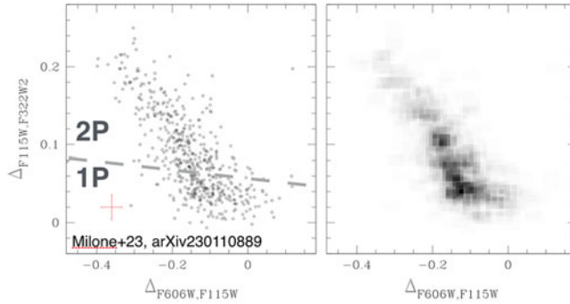
Figure 8. ChM from combined JWST- HST observations of 47 Tucanae M dwarfs (Milone et al. 2023). On the left panel the dashed line separates 1P from 2P stars. The right panel is the Hess diagram of the ChM. The expected error is represented in red on the left-side panel.
